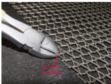
Making a Belt Splice Rod
