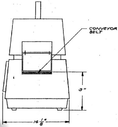
ENTRANCE ELEV
